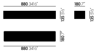
Caisson suspendu
